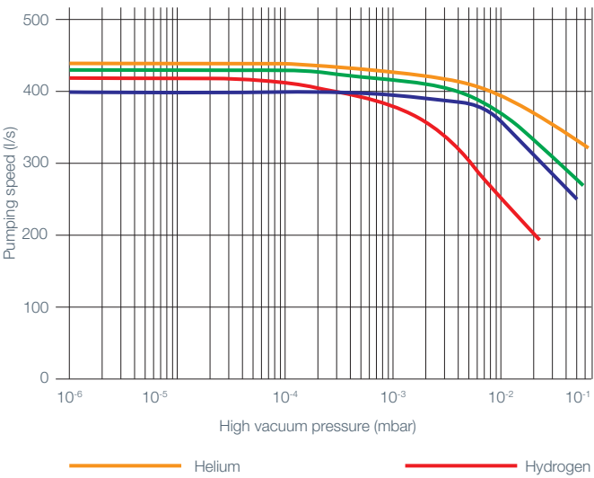
TURBOVAC 450 i/iX
