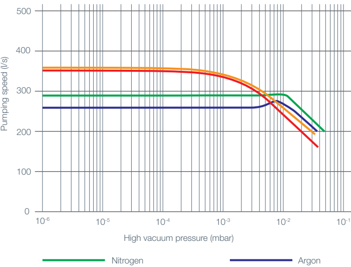
TURBOVAC 350 i/iX
