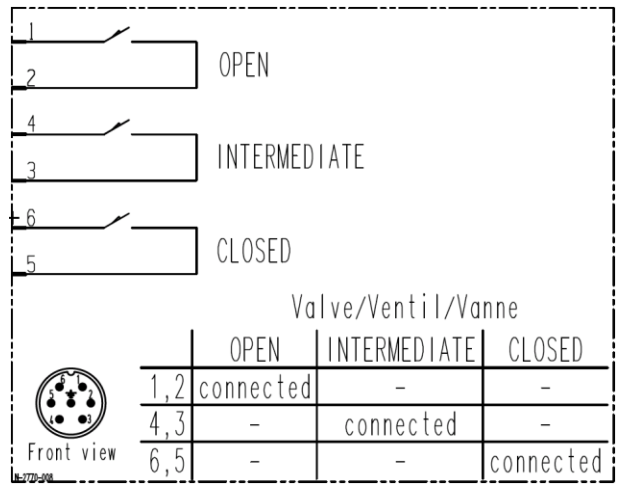
Wiring diagram
