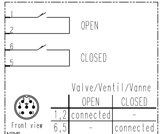
Wiring diagram
