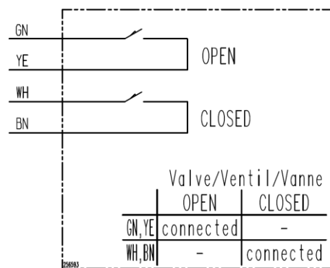
Wiring diagram
