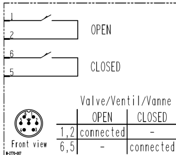
Wiring diagram
